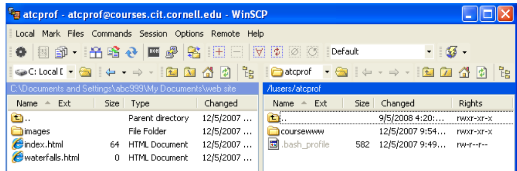
Figure 2 Main WinSCP Window.
